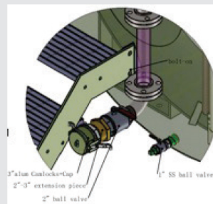
Liquip Farm Tank and fuel dispensing system
